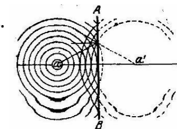
Fig. 306 Reflection of sound waves from \alpha at a wall AB and apparent generation of a new source of sound \alpha' (echo)
